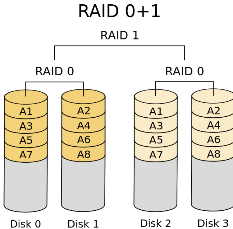
Figura 7: RAID 0+1.
