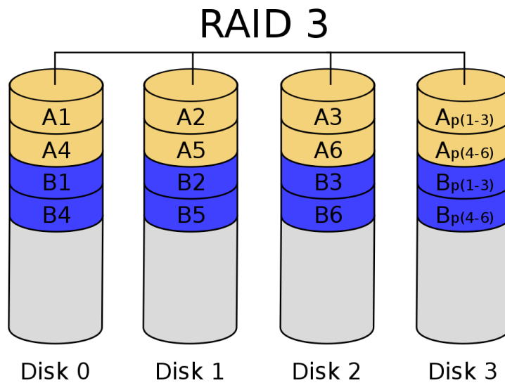
Figura 3: Diagram of RAID 3 setup.
