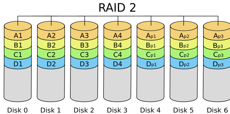
Figura 2: Diagram of RAID 2 setup.
